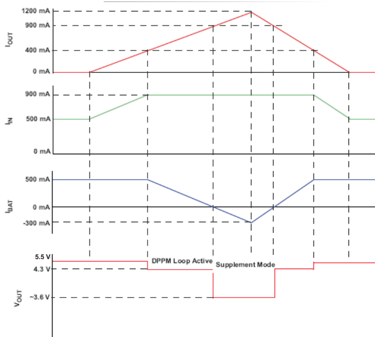
Figure 30. bq24075T, '79T DPPM and Battery Supplement Modes ( V_{\text{OREG}} = 5.5\text{V} , V_{\text{BAT}} = 3.6\text{V} )
