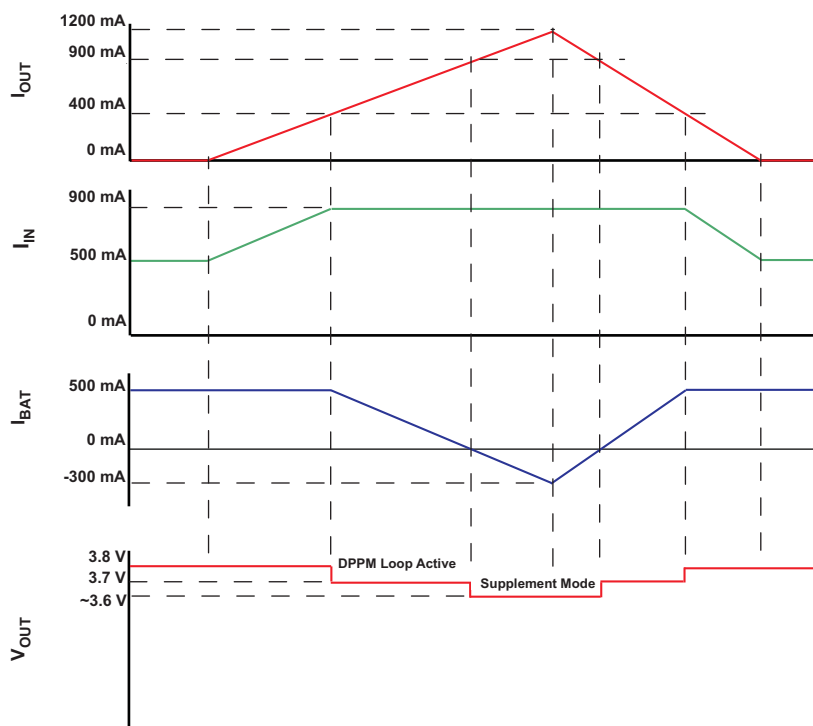
Figure 31. bq24072T DPPM and Battery Supplement Modes ( V_{\text{OREG}} = V_{\text{BAT}} + 225\text{mV} , V_{\text{BAT}} = 3.6\text{V} )
