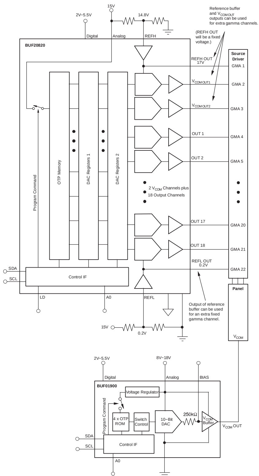
Figure 17. 22-Gamma Channel Solution
