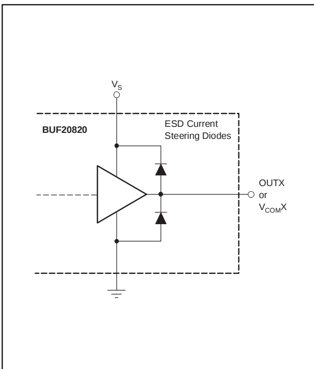
Figure 22. Output Pins ESD Protection Current-Steering Diodes
