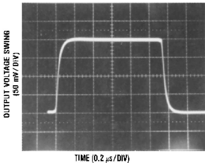
Figure 3. Small Signal Non-Inverting
