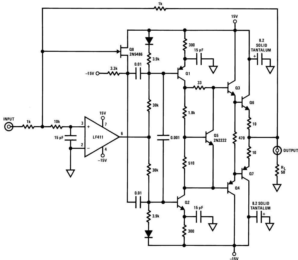
Figure 7. High Speed Current Booster
