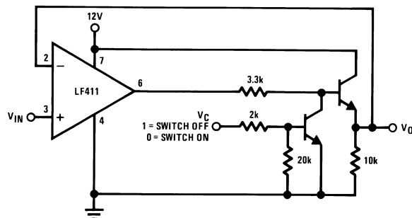
Figure 9. Single Supply Analog Switch with Buffered Output
