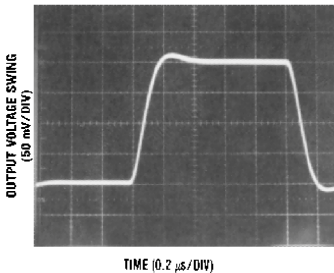
Figure 3. Small Signal Non-Inverting
