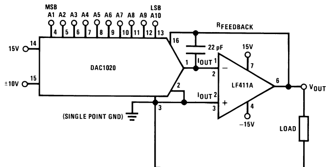
Figure 8. 10-Bit Linear DAC with No V_{OS} Adjust
