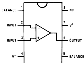
Figure 1. 8LD Ceramic Dual-in Line Package
