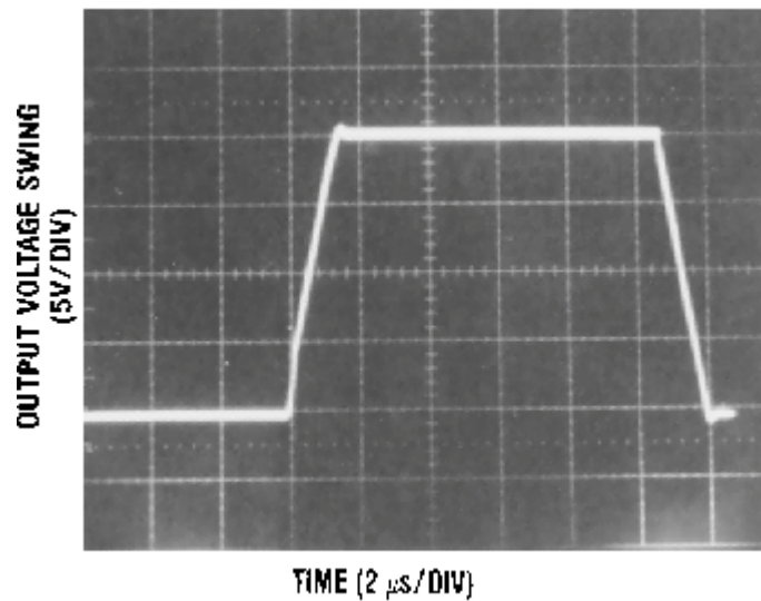
Figure 5. Large Signal Non-Inverting
