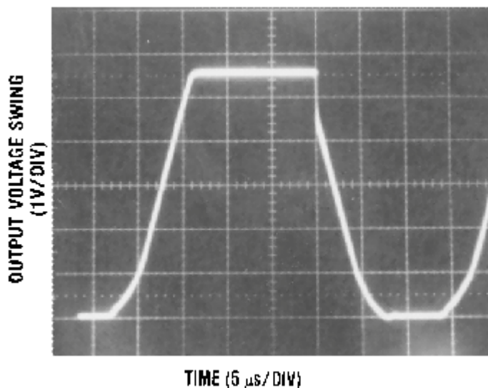
Figure 6. Current Limit ( R_L=100\Omega )
