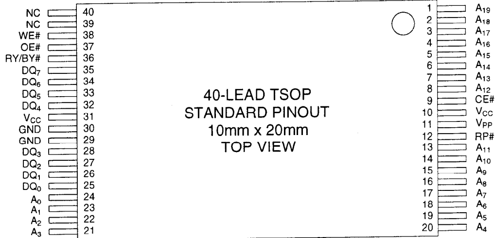
Figure 2. TSOP 40-Lead Pinout (Reverse Bend)
