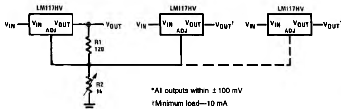
Adjustable Multiple On-Card Regulators with Single Control*
