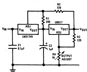
Tracking Preregulator
