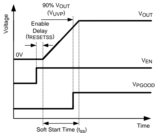
Figure 28. Soft Start Timing
