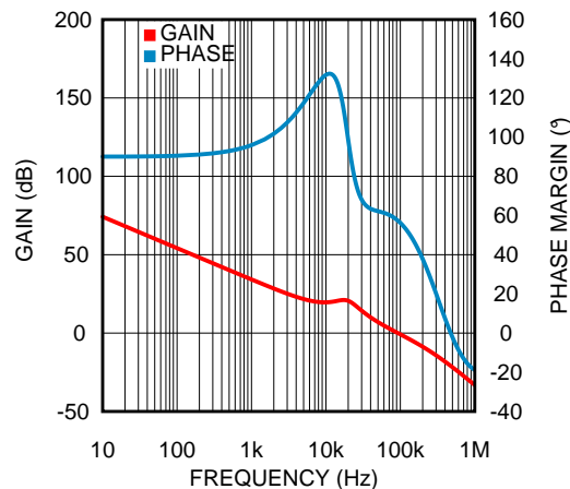
Figure 33. Loop Response
