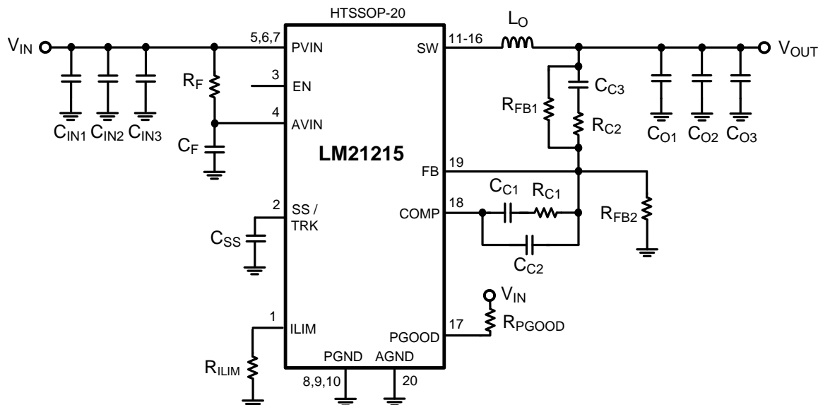
Figure 37. Typical Application Schematic 1
