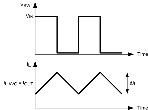
Figure 29. Switch and Inductor Current Waveforms
