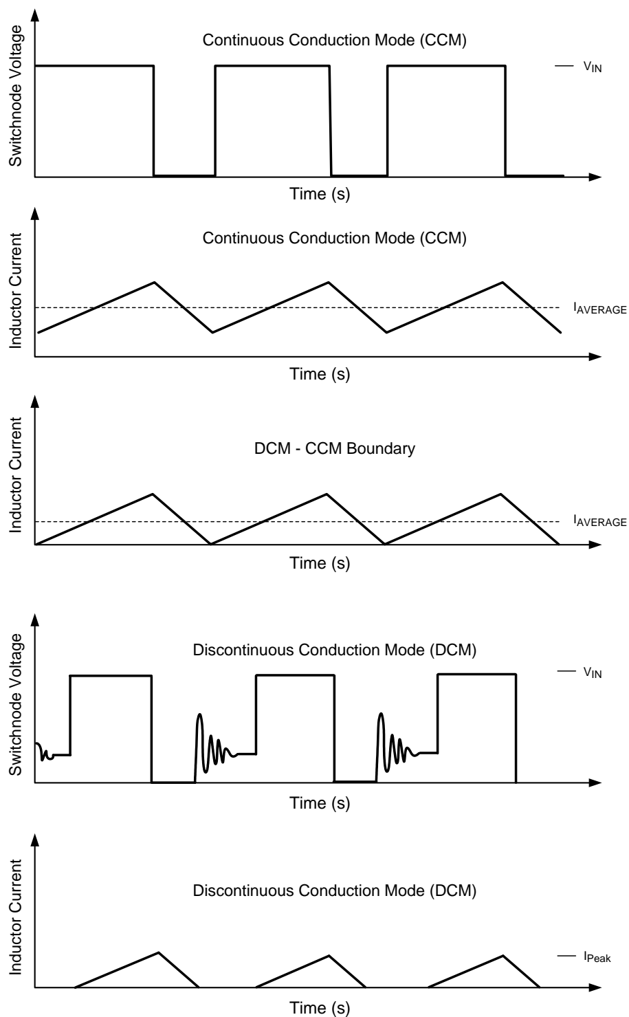
Figure 25. Modes of Operation for LM21215
