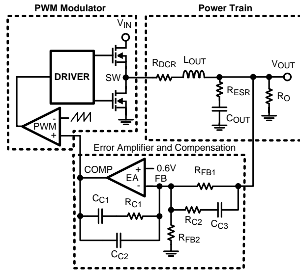
Figure 30. Loop Diagram
