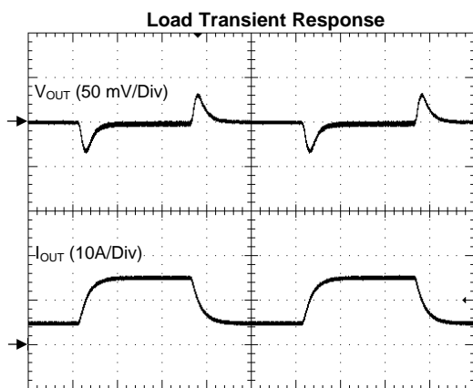
100 µs/DIV Figure 17.
