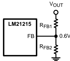
Figure 26. Setting V_{OUT}
