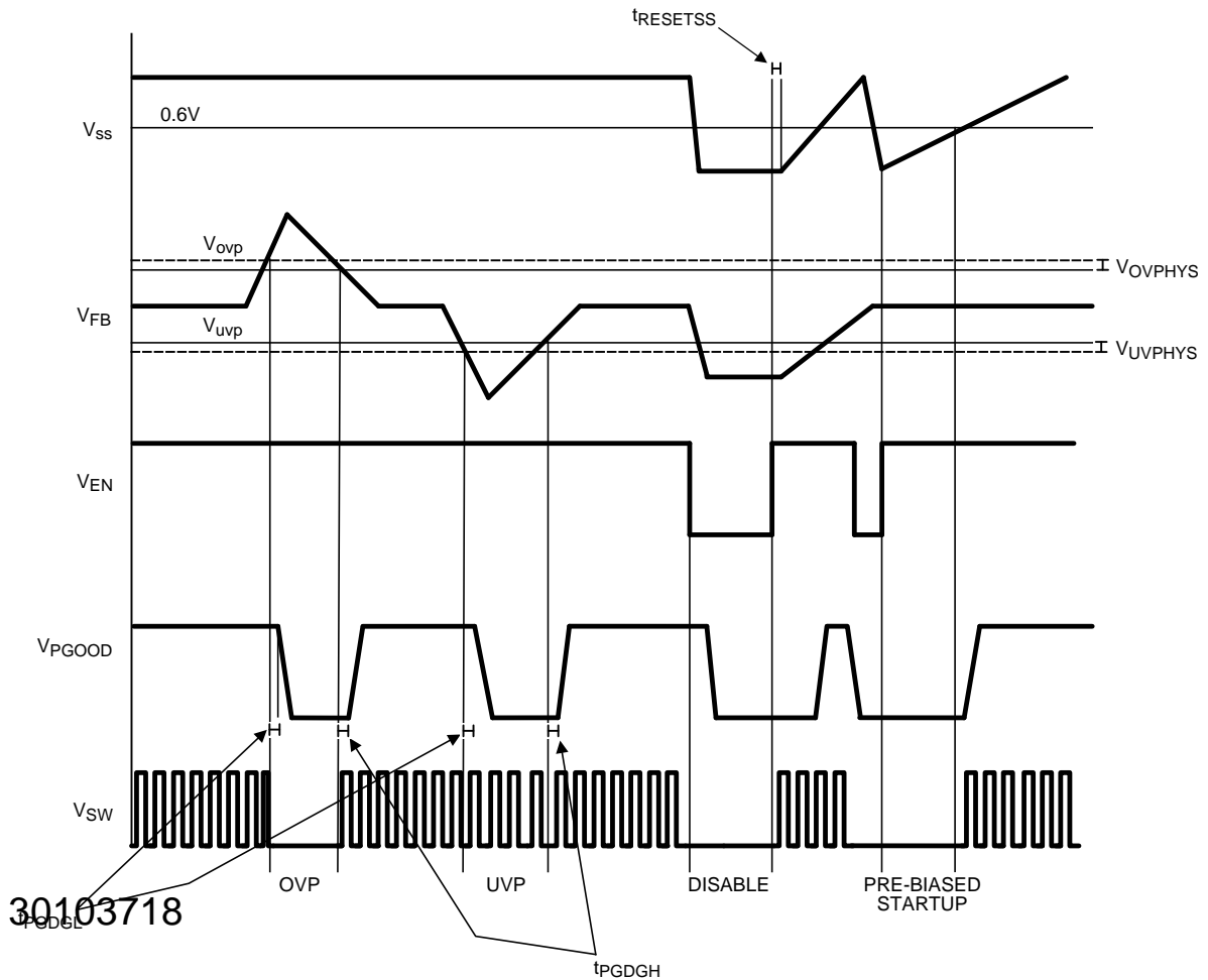
Figure 24. PGOOD Conditions
