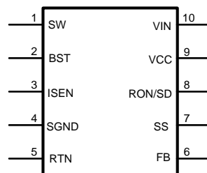
Figure 2. 10-Lead LLP
