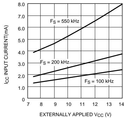
Figure 5. I_{CC} vs Externally Applied V_{CC}
