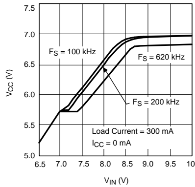
Figure 3. V_{CC} vs V_{IN}
