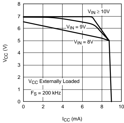
Figure 4. V_{CC} vs I_{CC}
