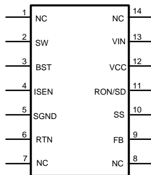
Figure 1. 14-Lead TSSOP
