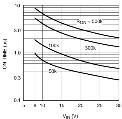
Figure 6. ON-Time vs V_{IN} and R_{ON}
