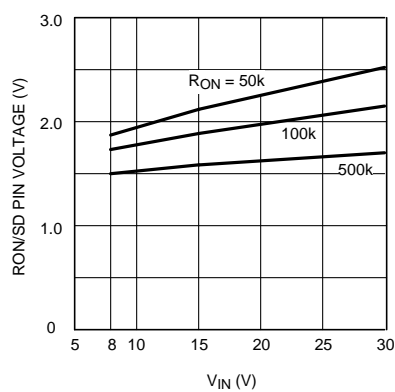
Figure 7. Voltage at R_{ON}/SD Pin
