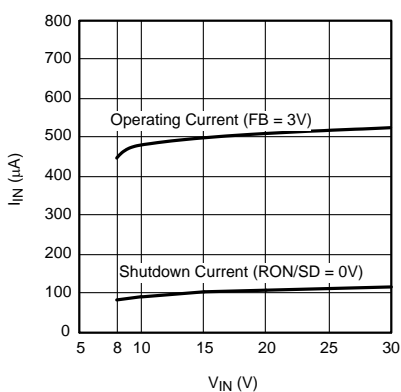
Figure 8. I_{IN} vs V_{IN}
