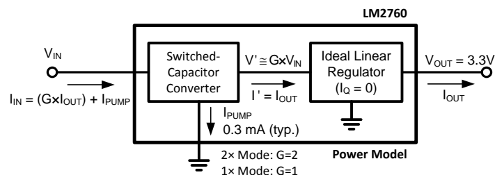
Figure 10. LM2760 Power Model
