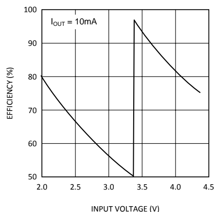
Figure 11. LM2760 Power Efficiency vs. Input Voltage ( T_A = 25^\circ C )
