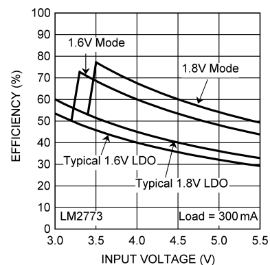
Figure 1. LM2773 Efficiency vs. Low-Dropout Linear Regulator (LDO) Efficiency
