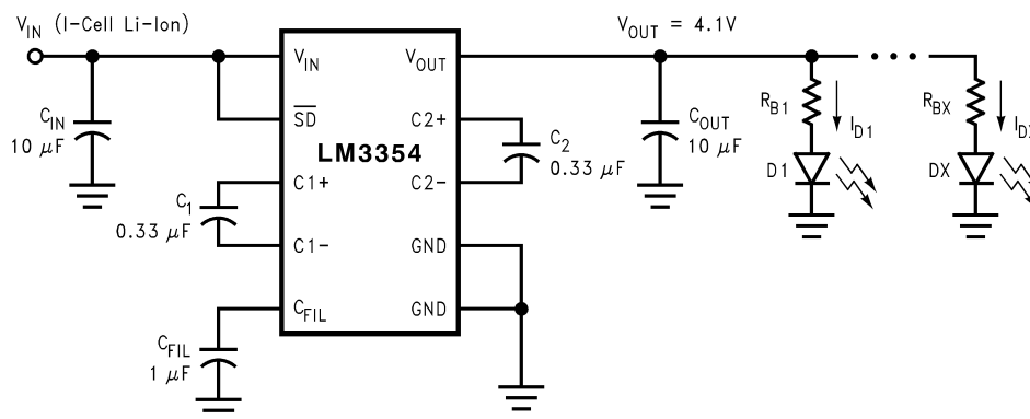
Figure 13. White LED Driver
