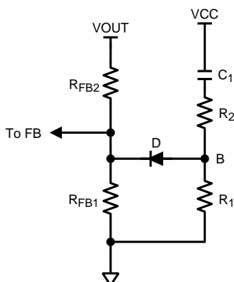
Figure 11. Soft-Start Circuit
