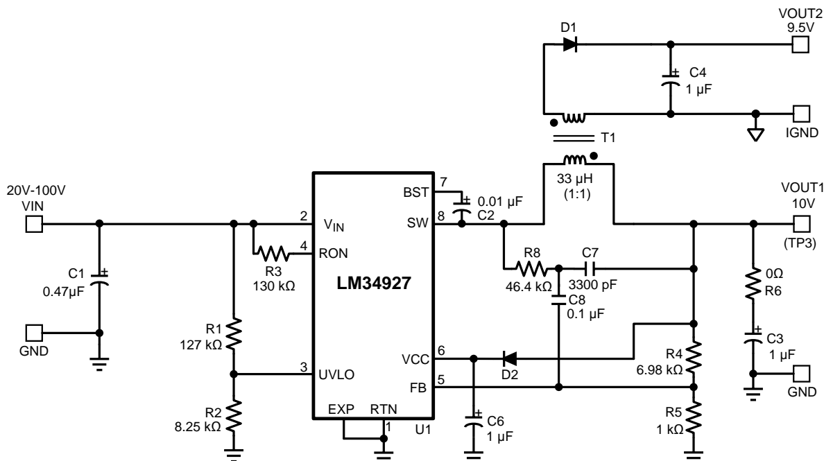
Figure 9. A 3W Isolated Application Schematic
