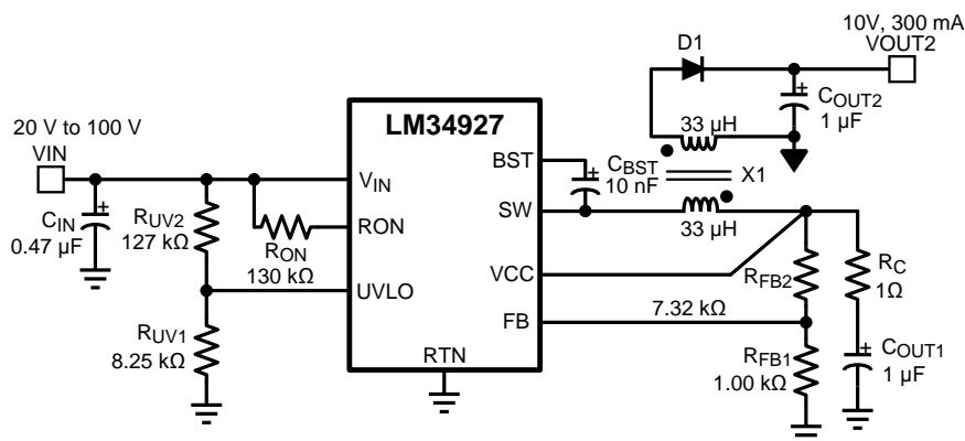
Figure 10. Lowest Part Count Isolated Application Schematic
