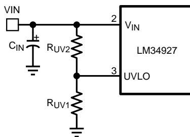
Figure 7. UVLO Resistor Setting
