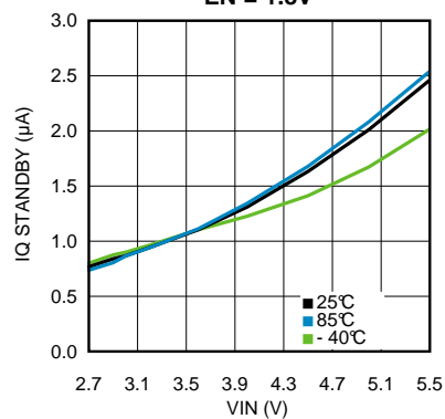
I_Q Standby vs. V_{IN} EN = 1.8V
