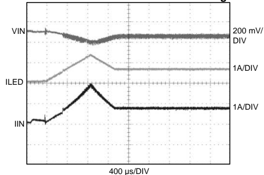
Input Voltage Flash Monitor, Up and Down Mode (0mV Hysteresis, 1/2 Step Filter Time)
