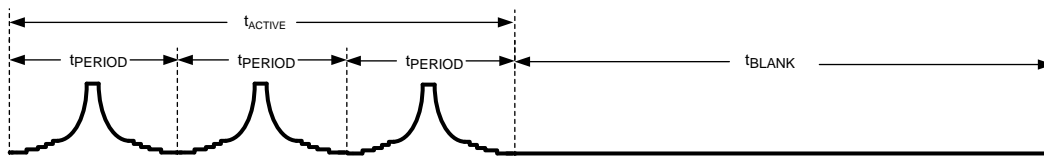
Figure 14. Multiple Pulse with Dead Time
