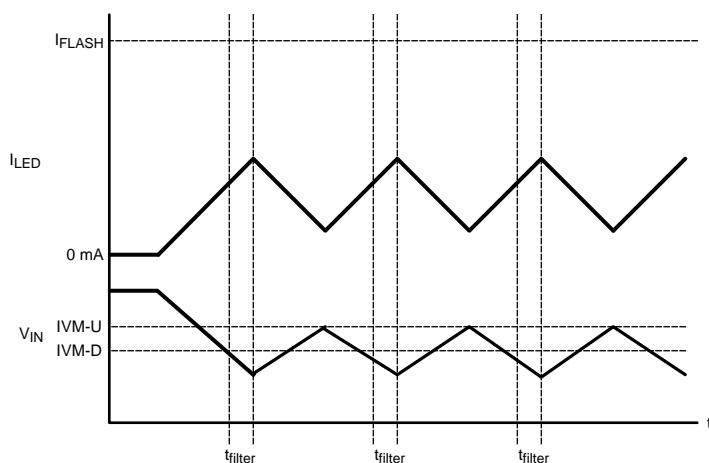
Figure 10. Adjust Up and Down Mode
