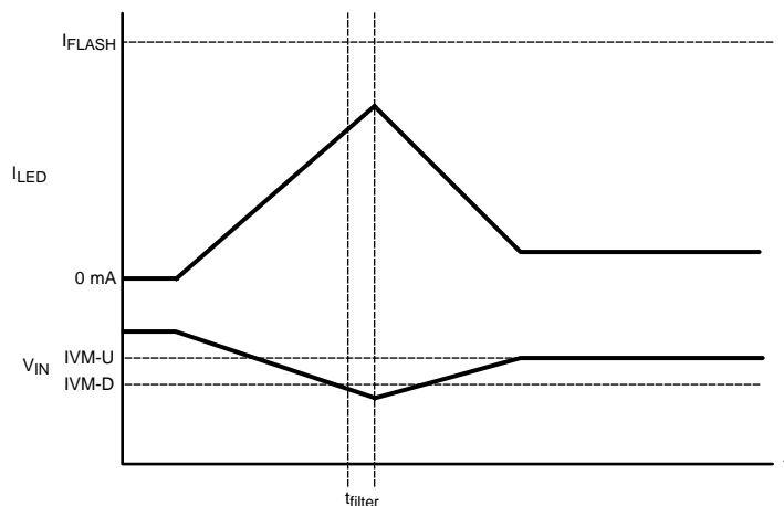
Figure 9. Adjust Down Only Mode
