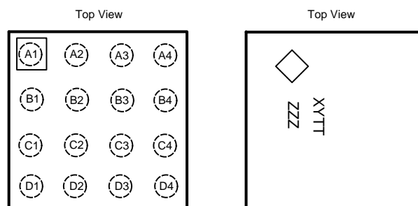
Figure 1. 16-Bump 1.615mm x 1.665mm x 0.6mm micro SMD Package YFQ16ACA XY (Date Code), TT(Die Traceability), ZZZ = D36 (Top Mark)
