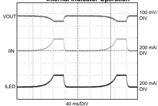
Internal Indicator Operation
