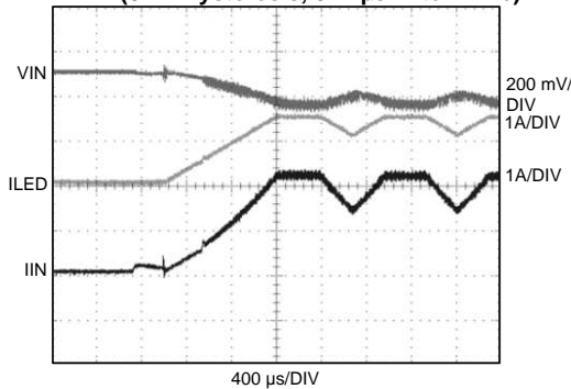
Input Voltage Flash Monitor, Up and Down Mode (0mV Hysteresis, 512 μs Filter Time)
