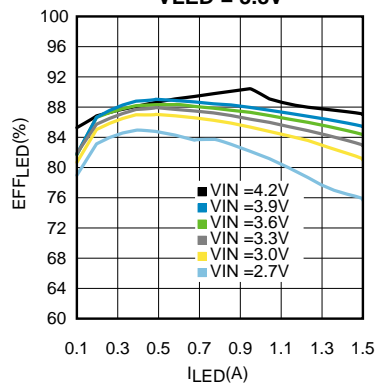
Torch LED Efficiency vs. V_{IN} V_{LED} = 3V
