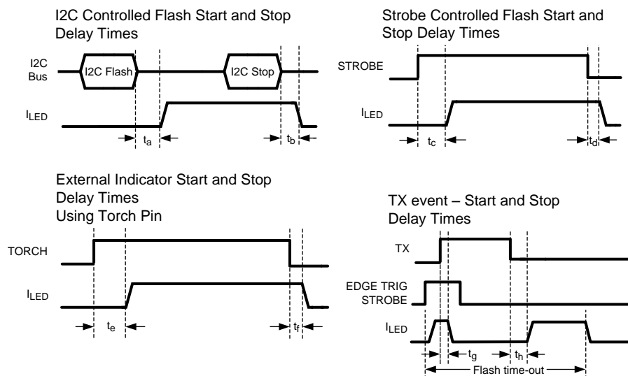
Figure 15. Control Logic Delays
