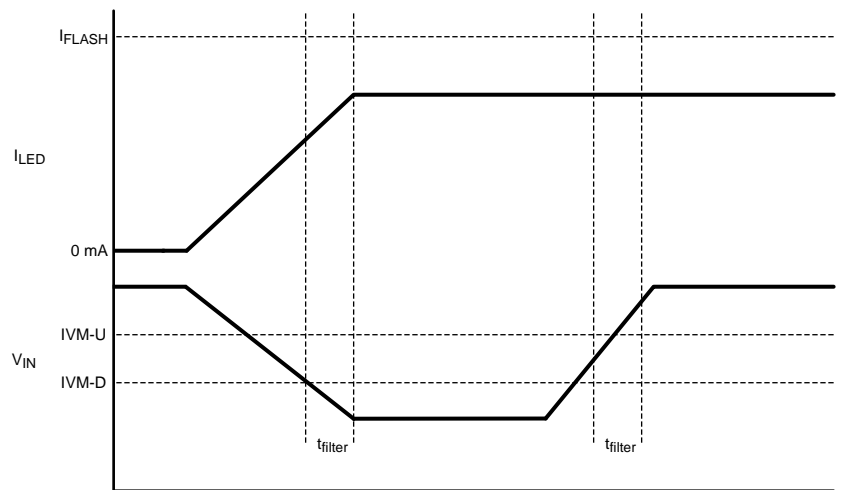
Figure 8. Stop and Hold Mode
