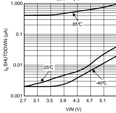
I_q Shutdown vs. V_{IN} EN = 0V
