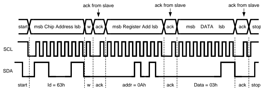
Figure 6. Write Cycle w = write (SDA = "0") r = read (SDA = "1") ack = acknowledge (SDA pulled down by either master or slave) id = chip address, 63h for LM3556
