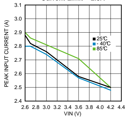
Input Current Limit Over-Temperature and V_{IN} Current Limit = 2.5A
