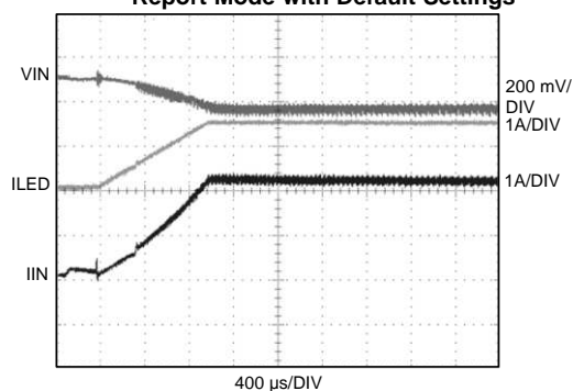
Input Voltage Flash Monitor Report Mode with Default Settings
