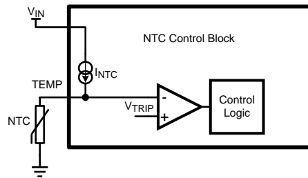
Figure 11. NTC Control Block
