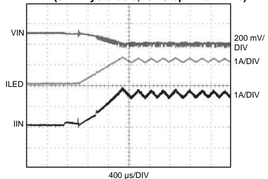
Input Voltage Flash Monitor, Up and Down Mode (256 μs Flash Ramp, 1/2 Step Filter Time)
