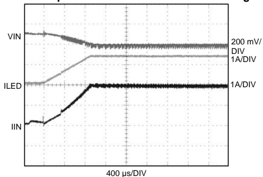
Input Voltage Flash Monitor Up and Down Mode with Default Settings
