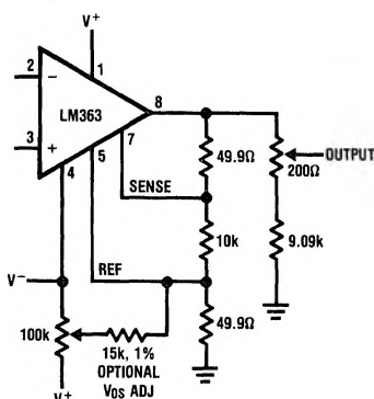
FIGURE 5. Adjusting Gain (8-Pin Package)
