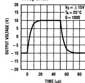
Large Signal Transient Response
