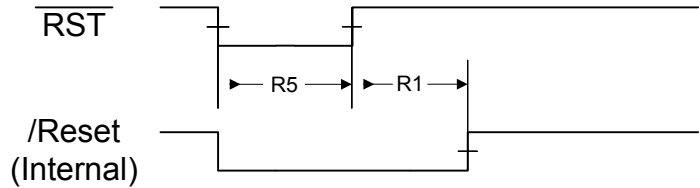
Figure 21-7. External Reset Timing ( \overline{RST} )
