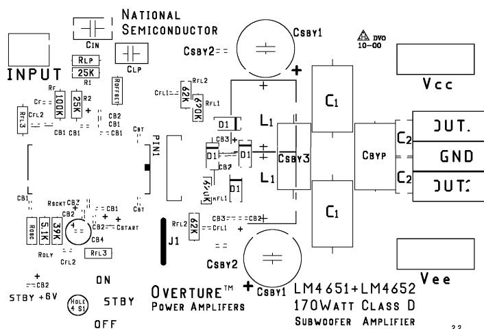
Figure 10. Reference PCB Silk Screen Layer
