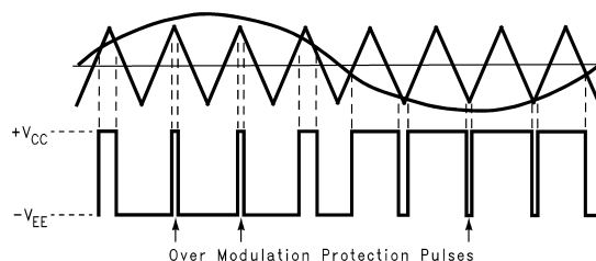
Figure 6. Over Modulation Protection
