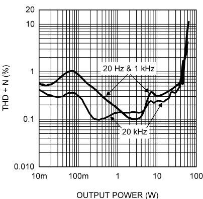
Figure 16. THD+N vs Output Power \pm 17V , f_{SW} = 175kHz R_L = 8\Omega , 30kHz BW
