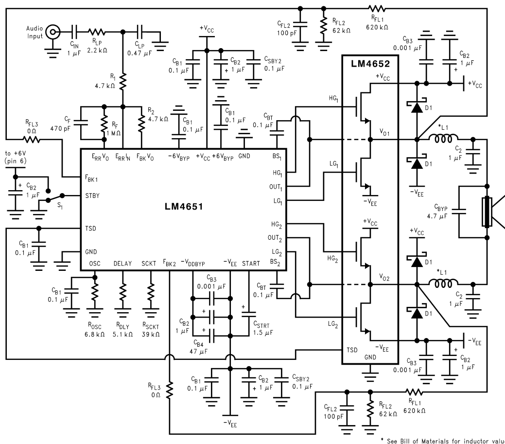
Figure 9. Reference PCB Schematic
