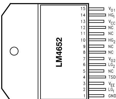
Figure 2. Isolated TO-220 Package Order Number LM4652TF See NS Package Number TF15B or Non-Isolated TO-220 Package Order Number LM4652TA See NS Package Number TA15A
