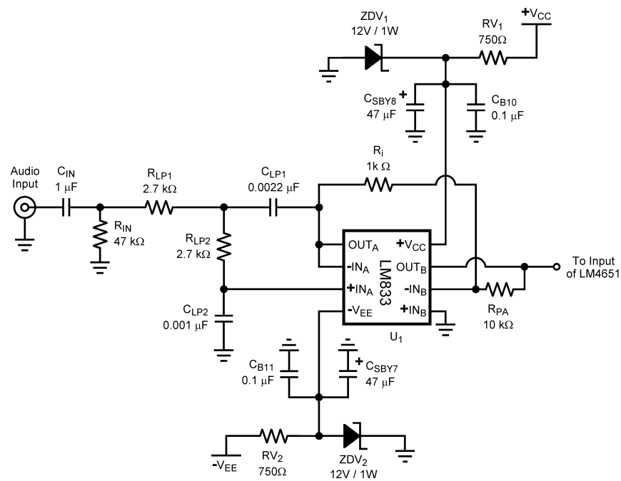
Figure 20. Input Pre-Amplifier And Filter Schematic
