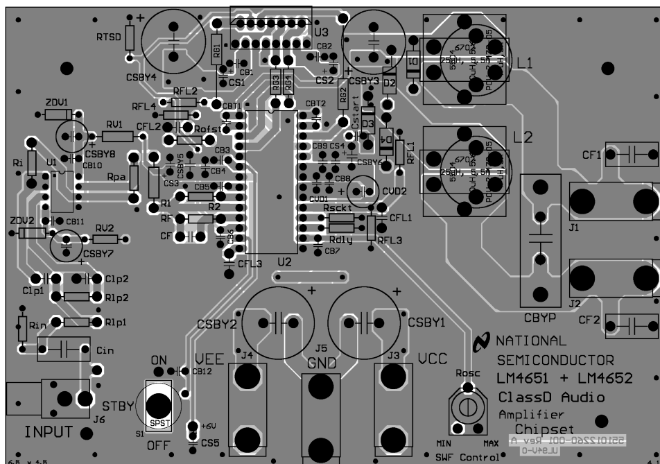
Figure 23. Composite Bottom View
