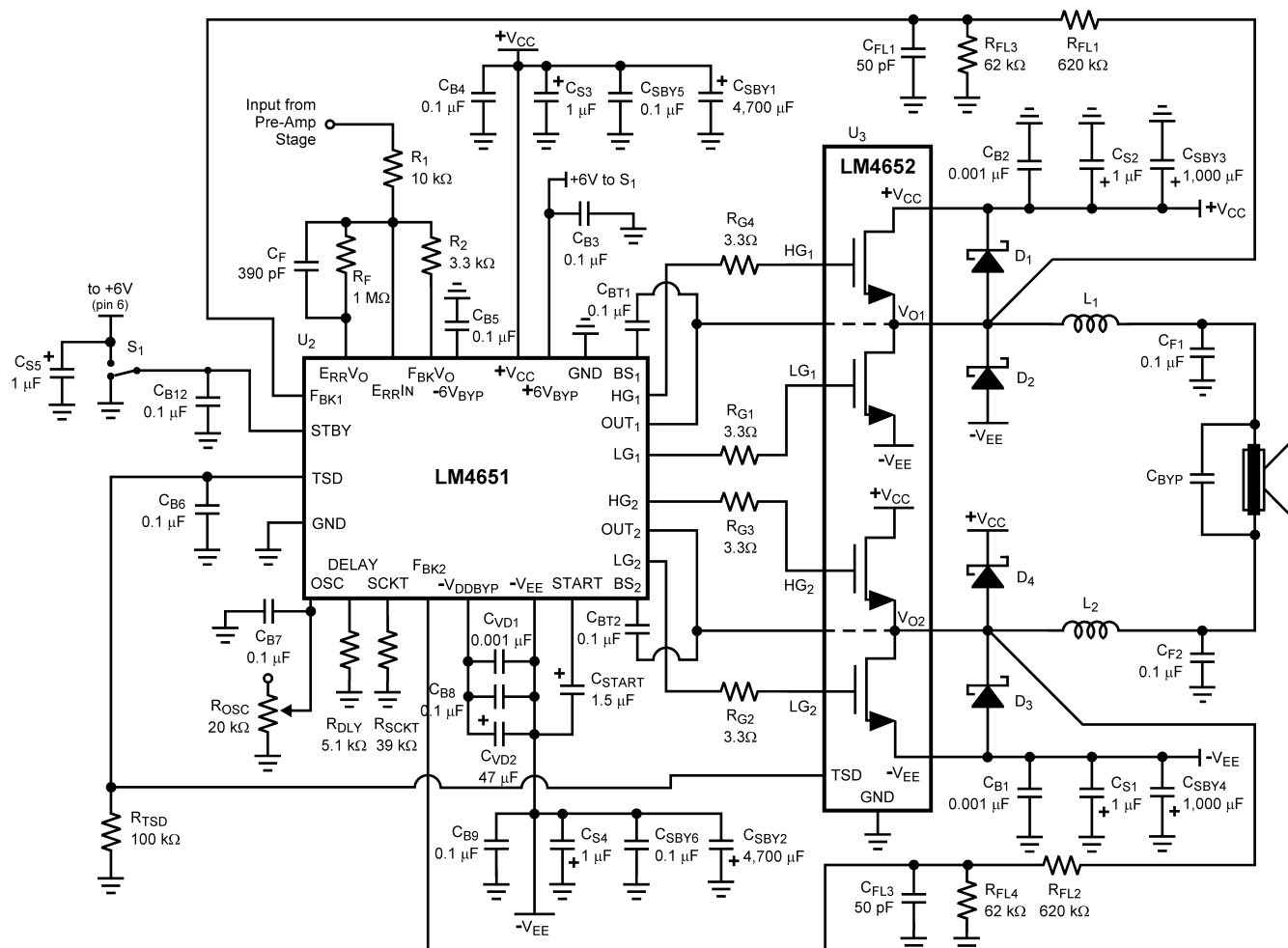
Figure 21. Full Audio Bandwidth Schematic
