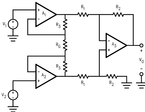
Figure 7. Feedback instrumentation Amplifier Schematic
