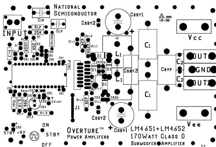
Figure 11. Reference PCB Silk Screen and Solder Mask Layers
