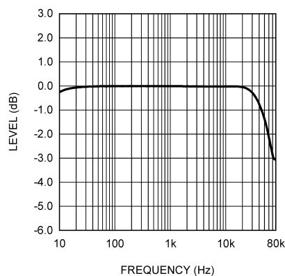
Figure 18. THD+N vs Frequency \pm 17\text{V} , f_{\text{SW}} = 175\text{kHz} , P_{\text{OUT}} = 1\text{W} \text{ \& } 50\text{W} R_L = 4\Omega , 30kHz BW
