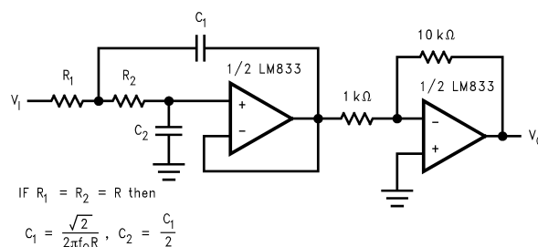
Figure 8. Pre-amplifier Stage with Low Pass Filter
