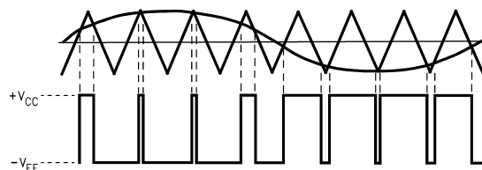
Figure 4. Conventional Pulse Width Modulation
