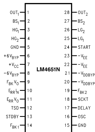
Figure 1. Top View Order Number LM4651N See NS Package Number N28B
