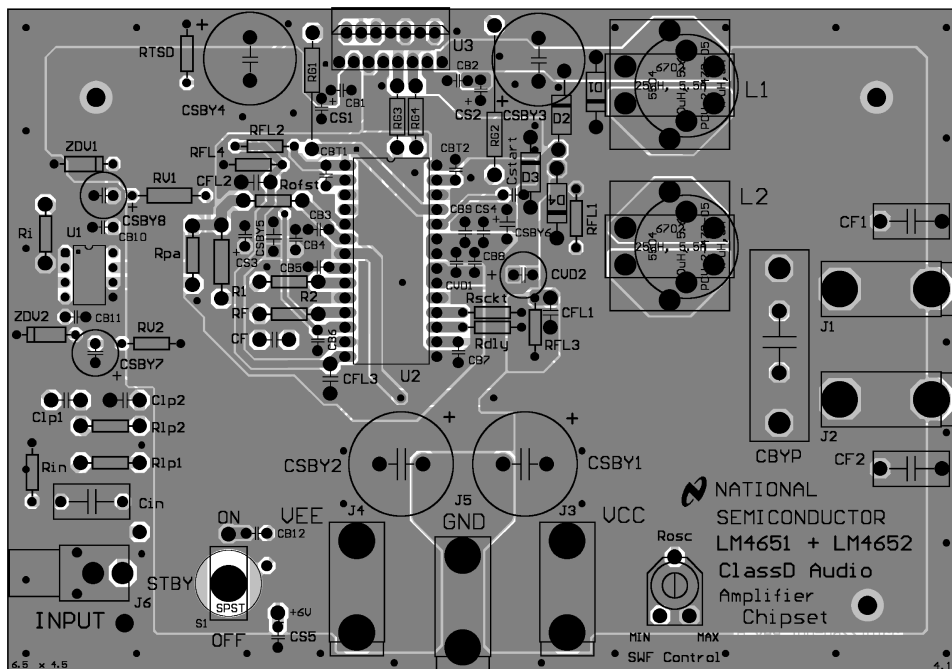
Figure 22. Composite Top View
