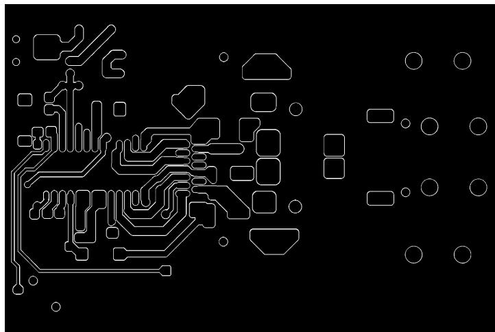
Figure 13. Reference PCB Bottom Layer
