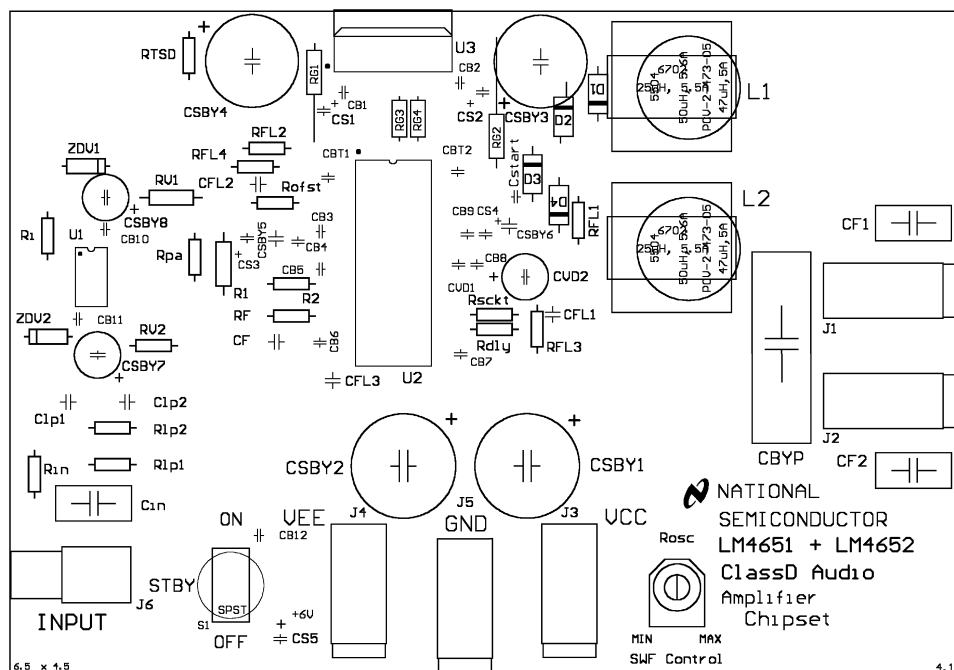
Figure 24. Silk Screen Layer
