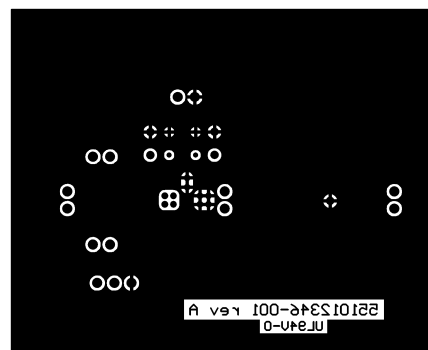
Figure 38. Bottom Layer
