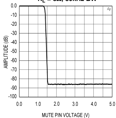
Mute Attenuation vs Mute Pin Voltage
