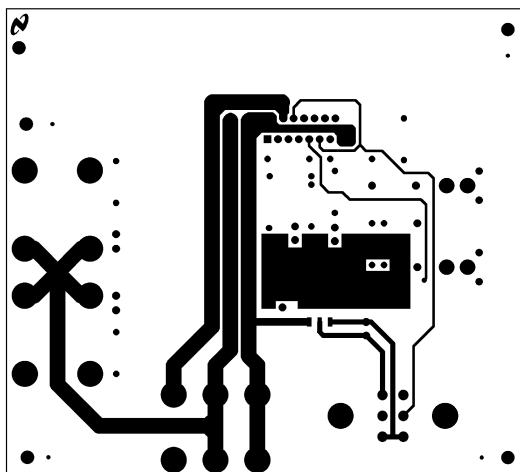
Figure 9. Top Layer
