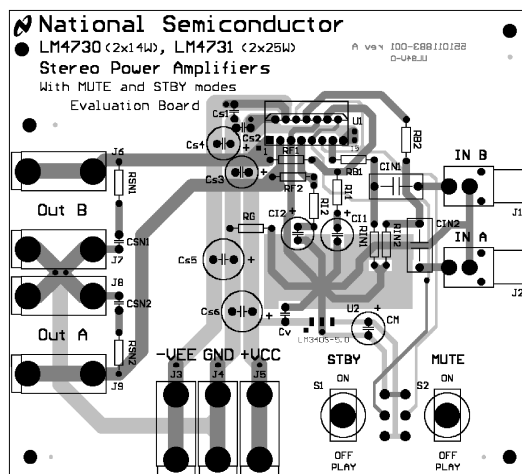
Figure 7. Composite View
