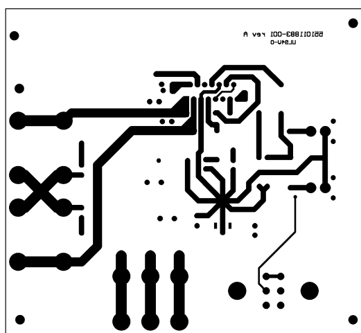
Figure 10. Bottom Layer
