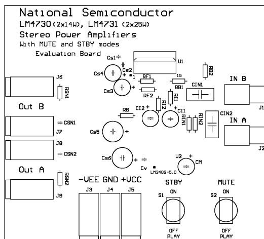
Figure 8. Silk Screen
