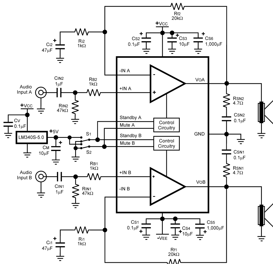
Figure 6. Reference PCB Schematic
