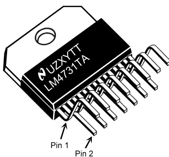
TO-220 Top Marking Top View
