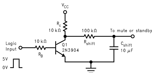
Figure 5. Level Shift Circuit
