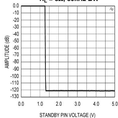
Standby Attenuation vs Standby Pin Voltage
