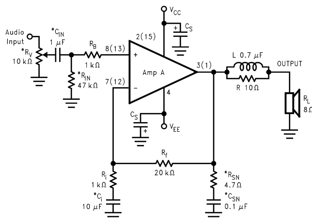
Figure 5. Special Audio Amplifier Application Circuit
