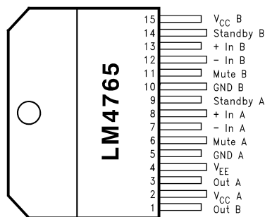
Figure 2. Plastic Package - Top View
