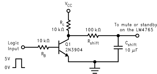
Figure 7. Level Shift Circuit
