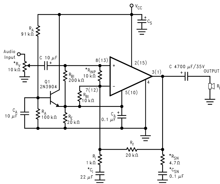
Figure 4. Single Supply Amplifier Application Circuit
