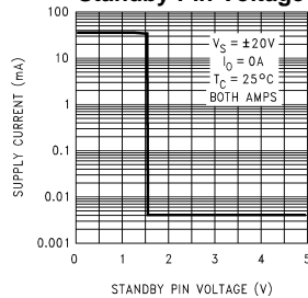
Supply Current ( I_{CC} ) vs Standby Pin Voltage
