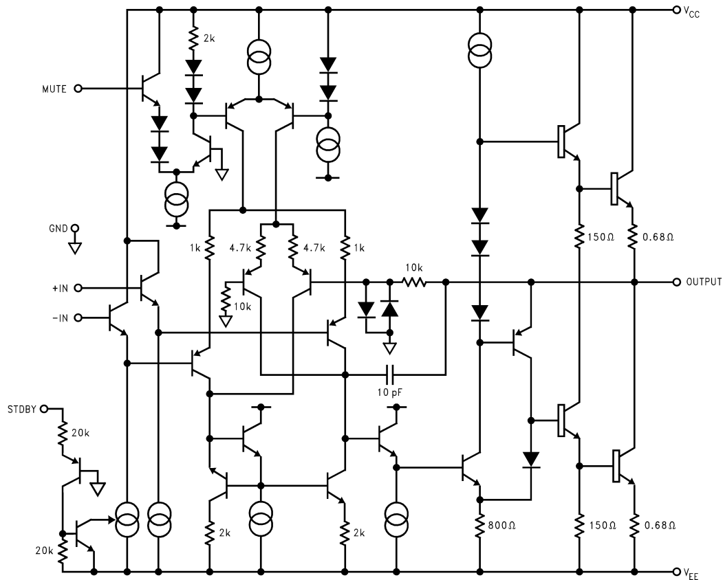
Figure 6. LM4765 (One Channel Only)
