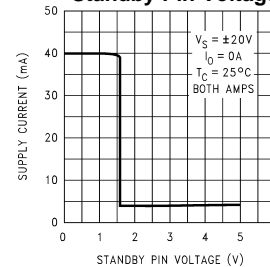
Supply Current ( I_{EE} ) vs Standby Pin Voltage
