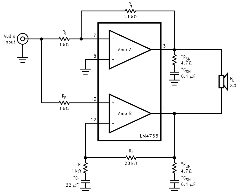
Figure 3. Bridged Amplifier Application Circuit
