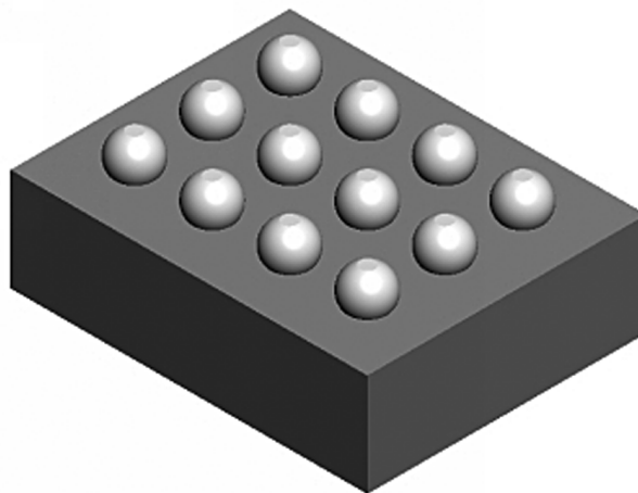
Figure 3. YZR0012 Package View (Bumps Up)
