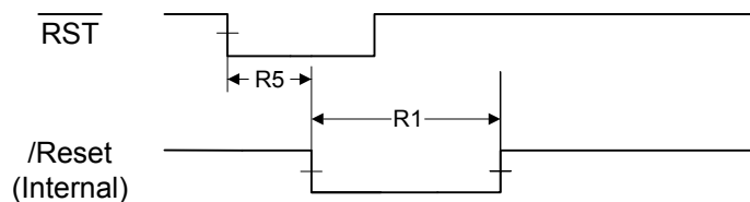
Figure 21-5. Software Reset Timing
