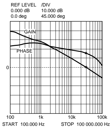
Figure 12. Overall Loop Gain and Phase
