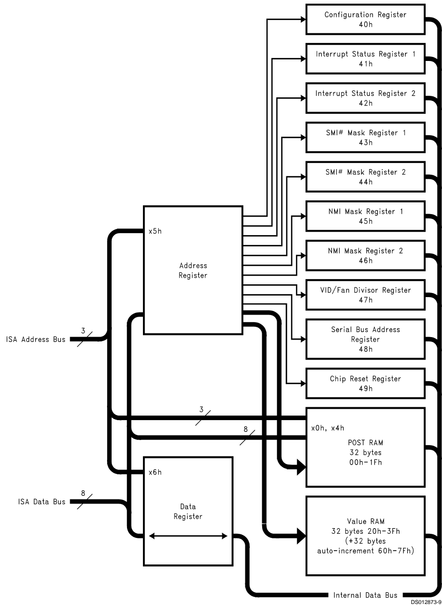
FIGURE 6. LM78 Register Structure
