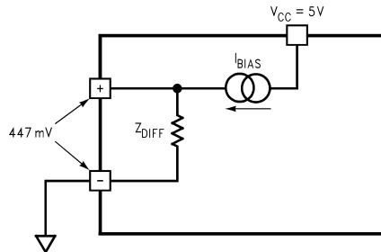
Figure 6. Equivalent Input Bias Circuit
