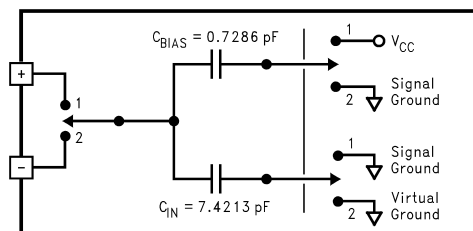
Figure 5. Simplified Switched Capacitor Input Circuit
