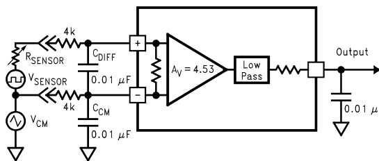
Figure 7. Differential and Common Mode Filtering
