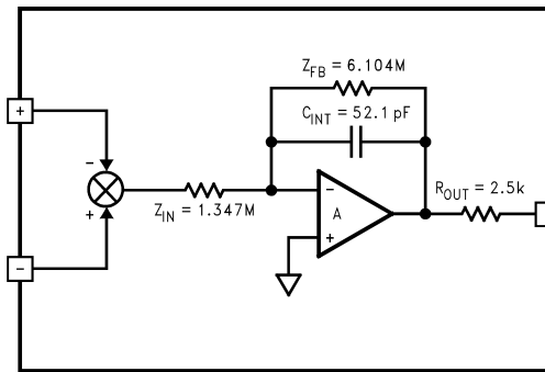
Figure 9. Equivalent Gain and Filter Circuit
