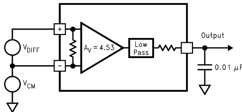
Figure 2. DC Test Circuit
