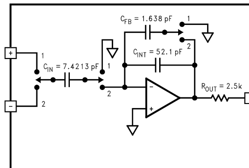
Figure 8. Simplified Gain and Filter Circuit
