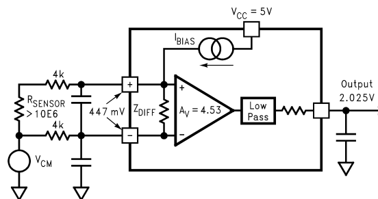
Figure 10. V_{OUT} with Cold Lambda Sensor
