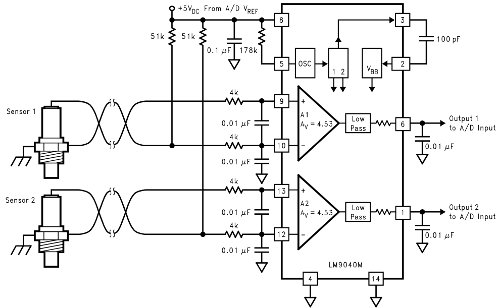
Figure 12. Typical Application
