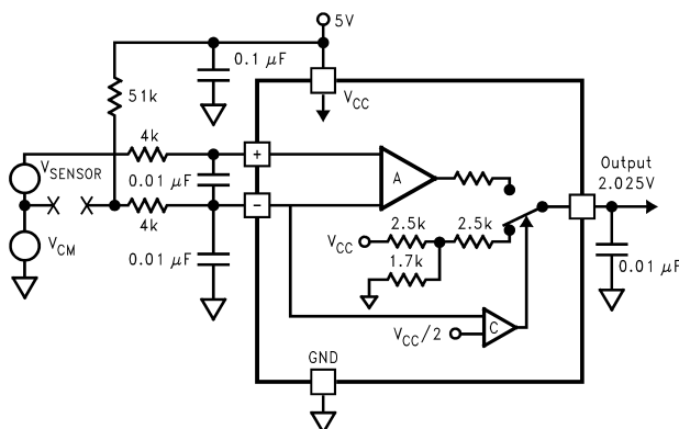
Figure 11. V_{OUT} with Open Inverting Input
