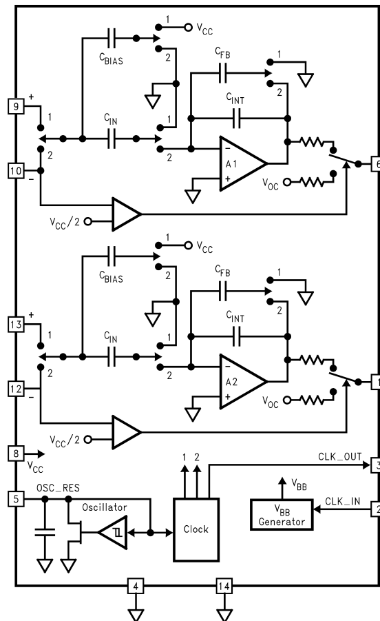
Figure 4. Simplified Circuit
