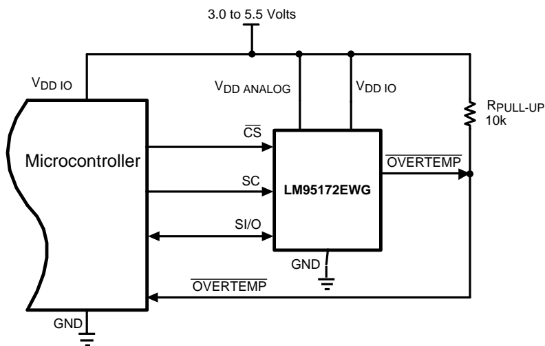
Figure 2. Microcontroller Interface - normal connection
