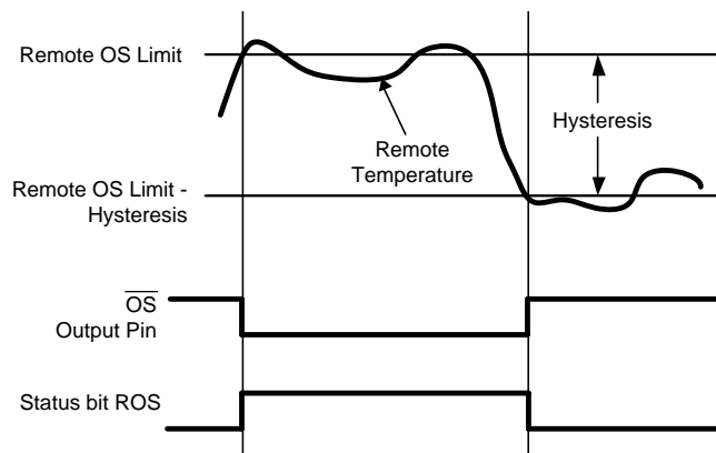
Figure 13. \overline{OS} Temperature Response Diagram
