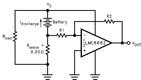
FIGURE 26b. Circuit Used to Sense Discharging
