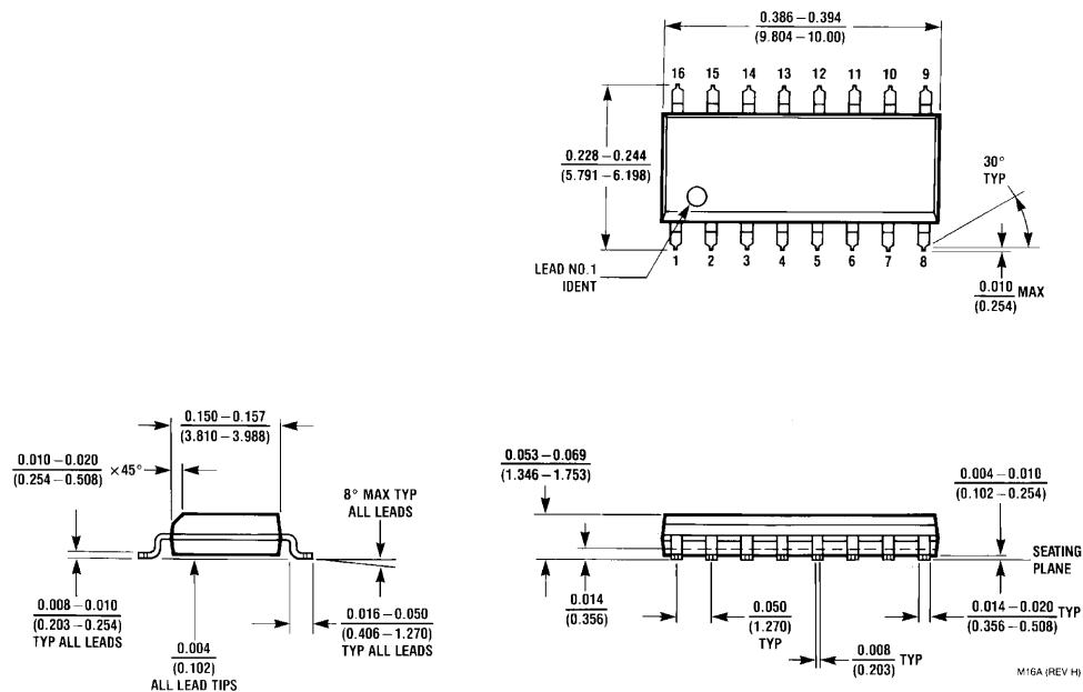
16-Pin Small Outline Package Order Number LMC6684AIM or LMC6684BIM NS Package Number M16A
