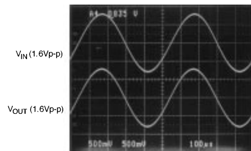
FIGURE 5. Response of the LMC6681/2/4 at V_S = 1.8V
