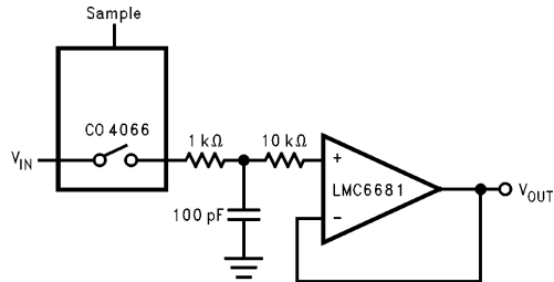
FIGURE 25. Sample-and-Hold Application
