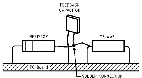
FIGURE 13. Air Wiring
