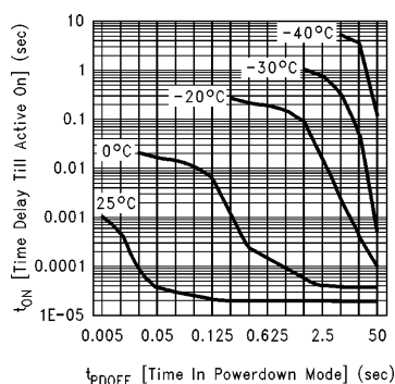
FIGURE 16. t_{ON} Delay Till Active-On after t_{PD OFF} in Powerdown Mode, V_S = 3V
