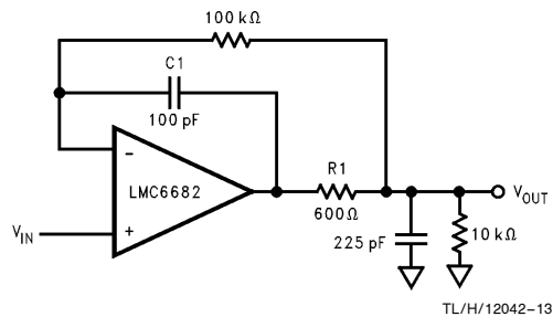
FIGURE 9. The LMC6682 Compensated to Ensure DC Accuracy and AC Stability
