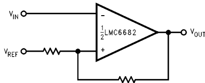
FIGURE 23. Comparator with Hysteresis
