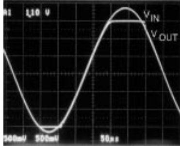
FIGURE 1. An Input Signal Exceeds the LMC6681/2/4 Power Supply Voltages with No Output Phase Inversion
