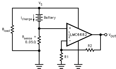
FIGURE 26a. Circuit Used to Sense Charging
