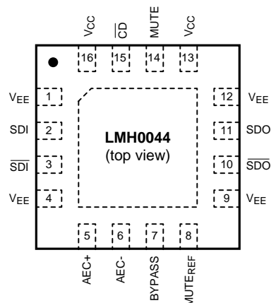
Figure 1. 16-Pin LLP Order Number LMH0044SQ See NS Package Number SQB16A
