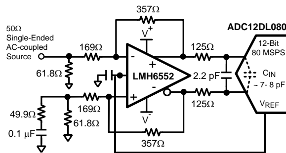
Figure 50. Driving a 12-bit ADC
