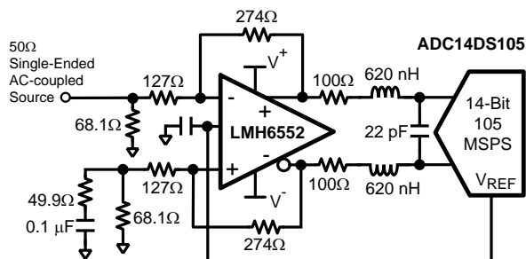
Figure 52. Driving a 14-bit ADC
