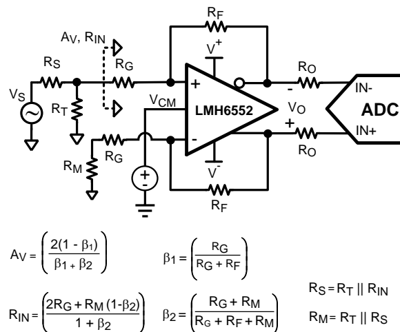
Figure 46. Single Ended Input with Differential Output
