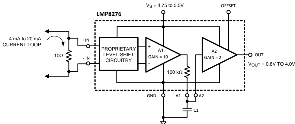
Figure 10. Current Loop Receiver
