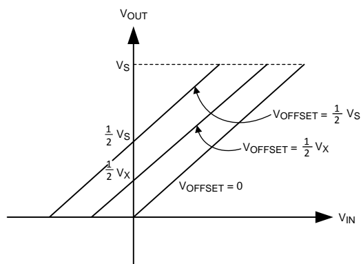
Figure 4. Mid-Rail Offset Adjustment Pin Function
