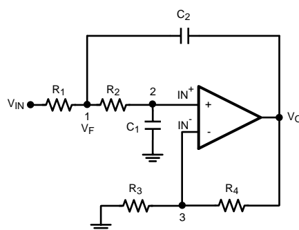
Figure 6. Second Order Low-Pass Filter
