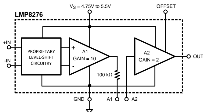
Figure 3. LMP8276
