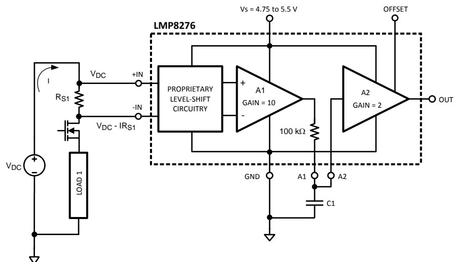
Figure 11. High Side Current Sensing
