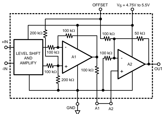
Figure 5. Mid-Rail Offset Adjustment Pin Schematic
