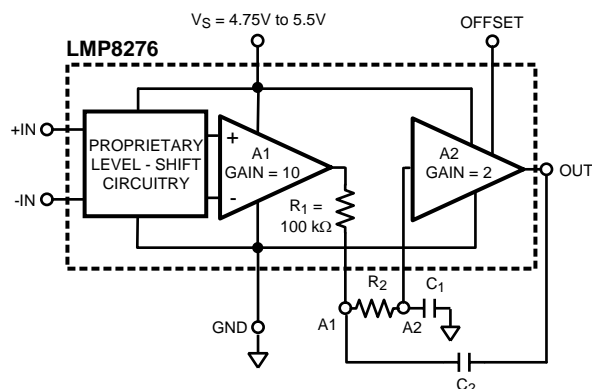
Figure 7. Low-Pass Filter With LMP8276
