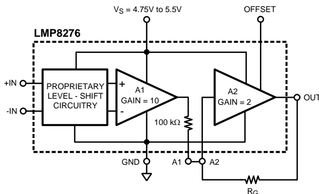
Figure 9. Gains Greater Than 20
