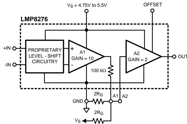
Figure 8. Gains Less Than 20
