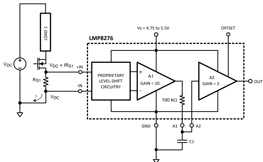
Figure 12. Low Side Current Sensing
