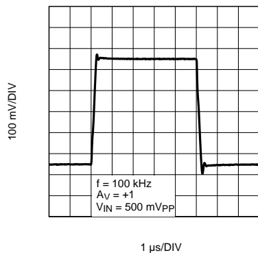
Large Signal Step Response with Gain = 1
