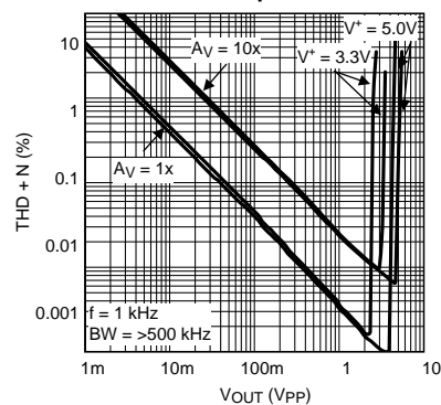
THD+N vs. Amplitude
