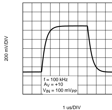
Large Signal Step Response with Gain = 10
