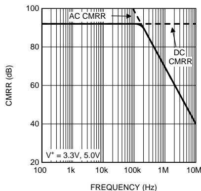
Figure 6. CMRR Curve
