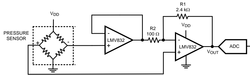
Figure 11. Pressure Sensor Application
