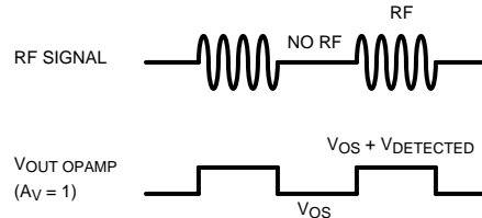
Figure 8. Offset voltage variation due to an interfering RF signal
