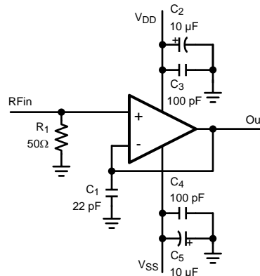
Figure 6. Circuit for coupling the RF signal to IN+
