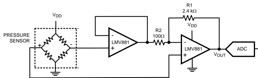
Figure 8. Pressure Sensor Application
