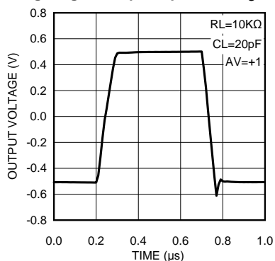
Large Signal Step Response at V_s = 3.3\text{V}
