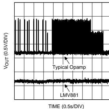
Figure 7. Comparing EMI Robustness
