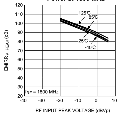
EMIRR IN+ vs. Power at 1800 MHz
