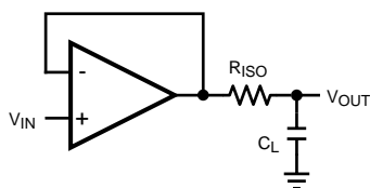
Figure 4. Isolating Capacitive Load
