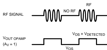
Figure 5. Offset voltage variation due to an interfering RF signal
