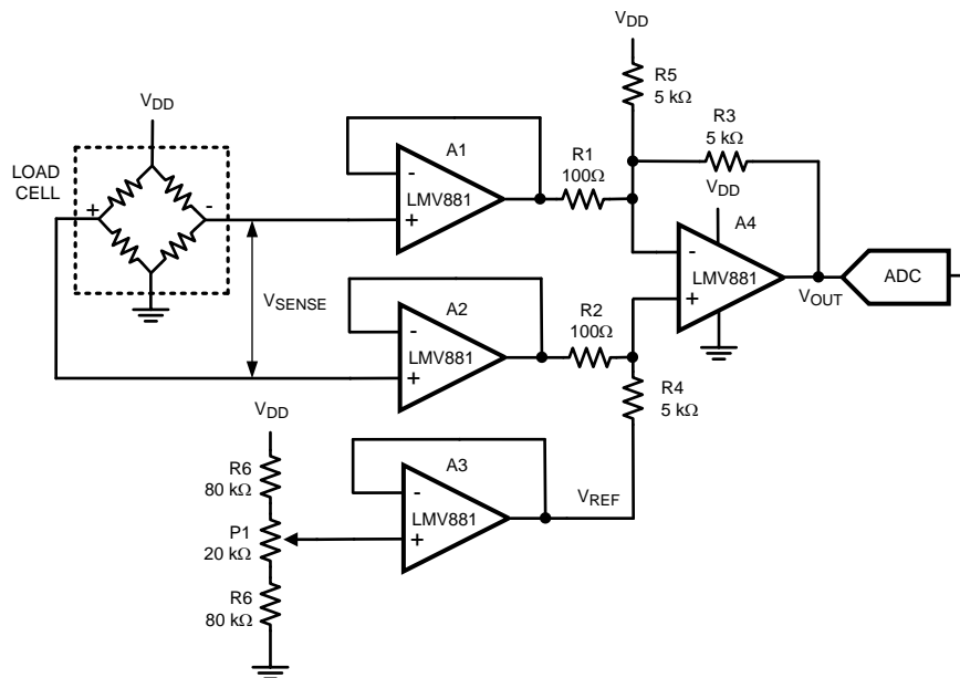
Figure 9. Load Cell Application
