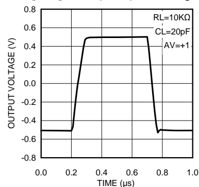
Large Signal Step Response at V_s = 5\text{V}
