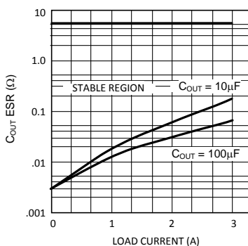
Figure 21. Minimum ESR vs Output Load Current
