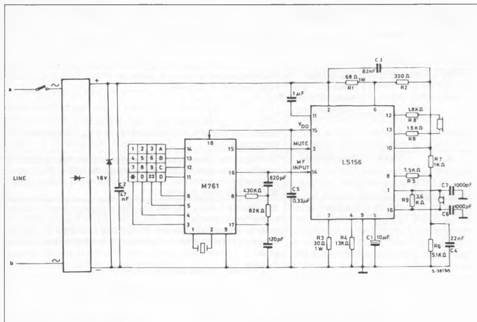
Figure 9 : Application Circuit with Multifrequency (EUROP I std.).
