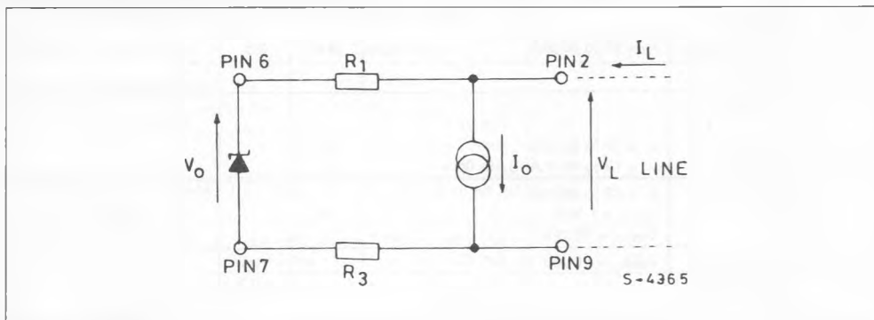
Figure 6 : Circuit Configuration of the Shunt Regulator.
