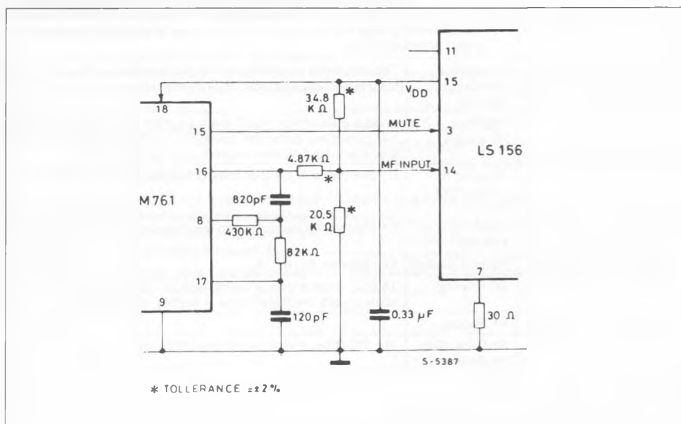
Figure 9 : Application Circuit with Multifrequency (EUROP I std.).
