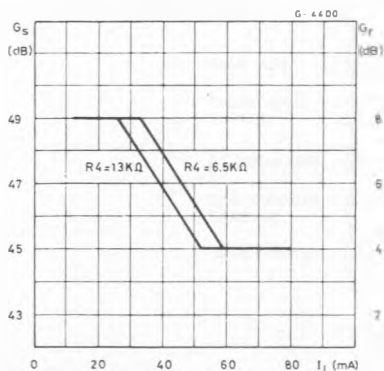
Figure 12 : Sending and Receiving Gain vs. Line Current.
