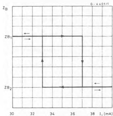
Figure 13 : Balance Network Impedance vs. Line Current.
