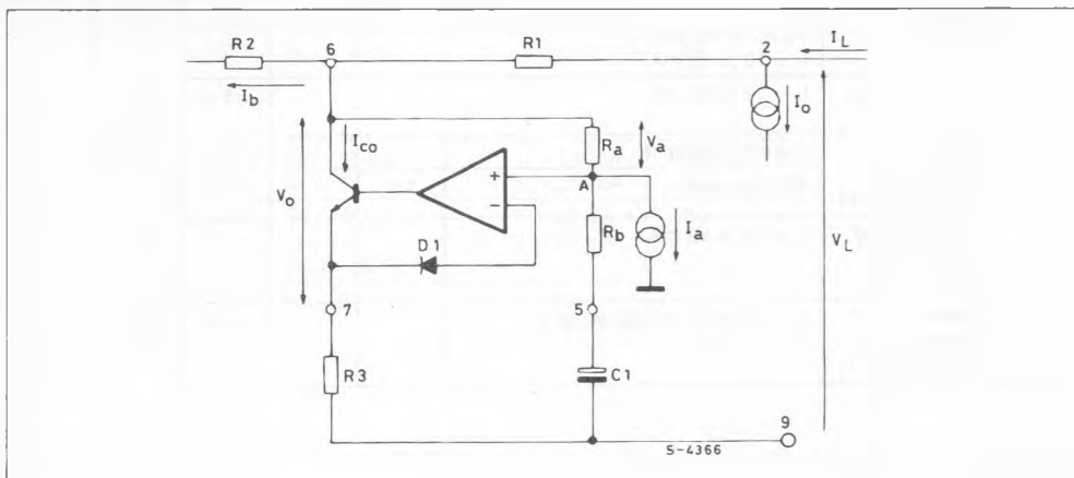
Figure 6 : Circuit Configuration of the Shunt Regulator.
