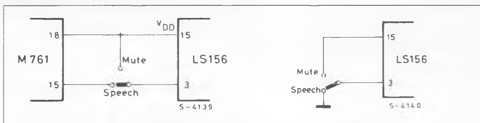
Figure 11 : Application Circuit without Multifrequency.
