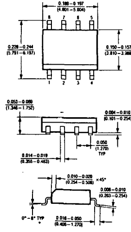
SO Package 8-Lead Plastic SOIC
