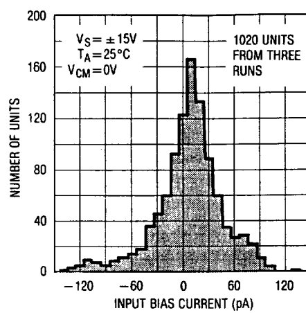
Typical Distribution of Input Bias Current
