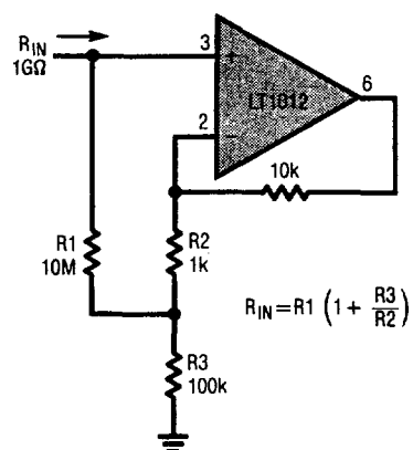
Resistor Multiplier
