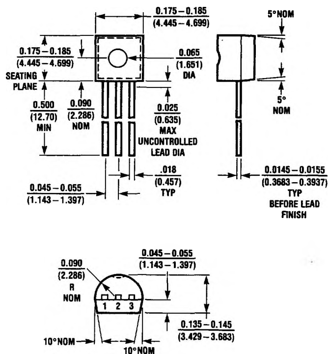
Z Package T0-92 Plastic
