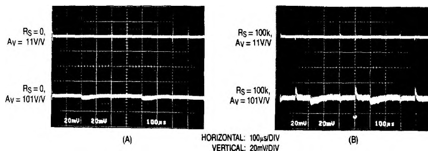
Figure 2. Clock Feedthrough
