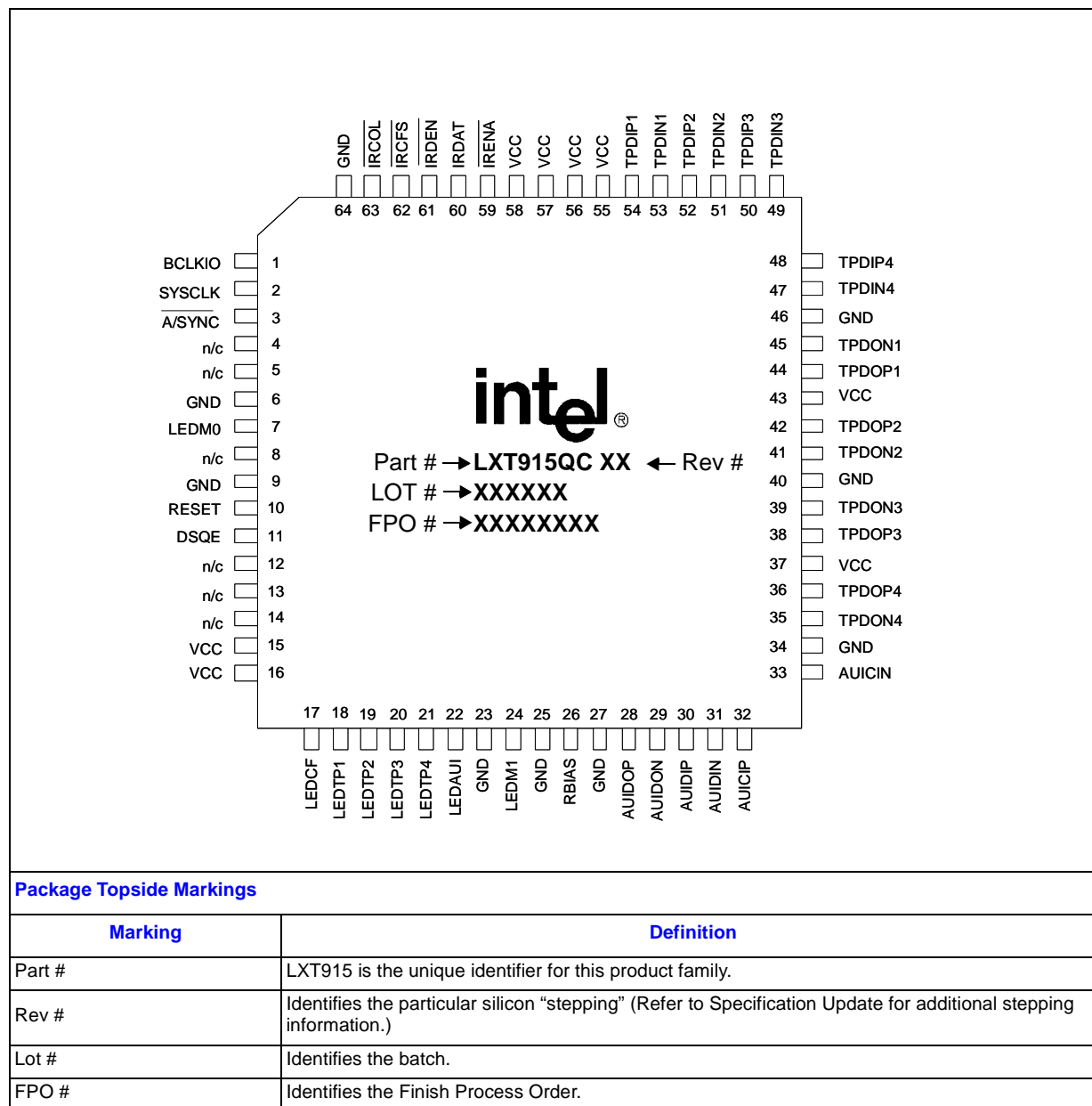
Figure 2. LXT915 Pin Assignments
