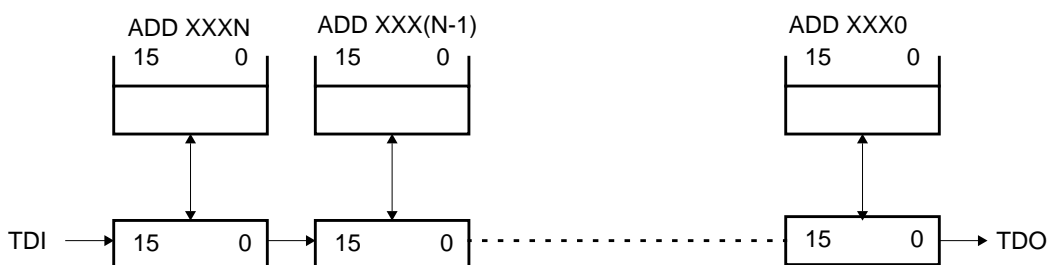
Figure 84. Bit Allocation Arrangement
