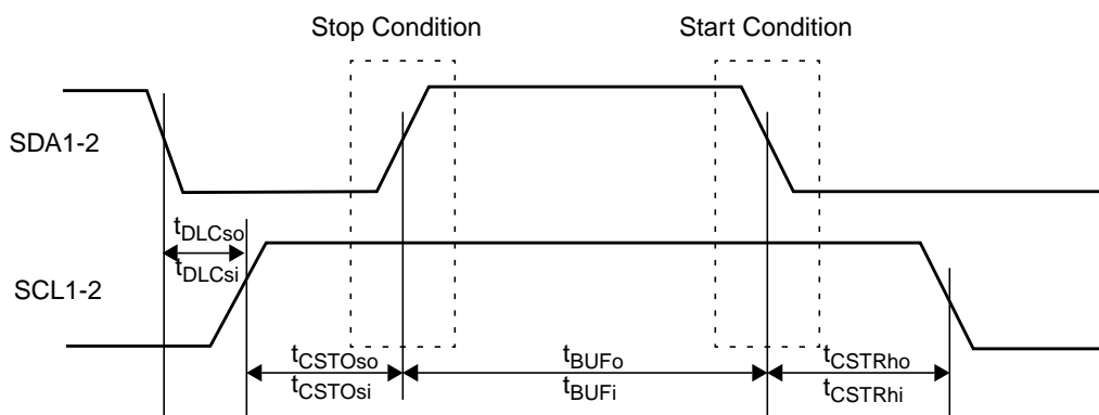
Figure 148. ACB Start and Stop Condition Timing
