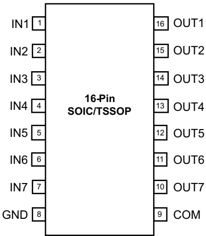
Figure 1. ULN2003LV PINOUT
