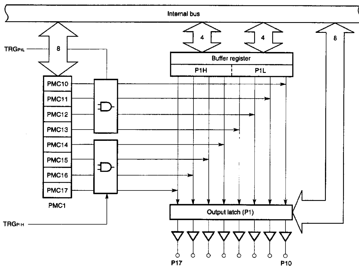
Fig. 3-6 Block Diagram of RTP1
