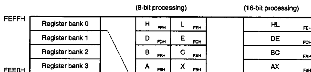
Fig. 2-6 Configuration of General Register
