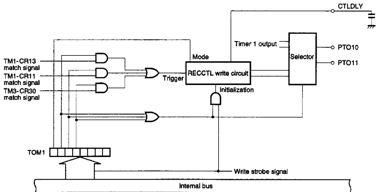
Fig. 3-18 Block Diagram of the RECCTL Write Circuit
