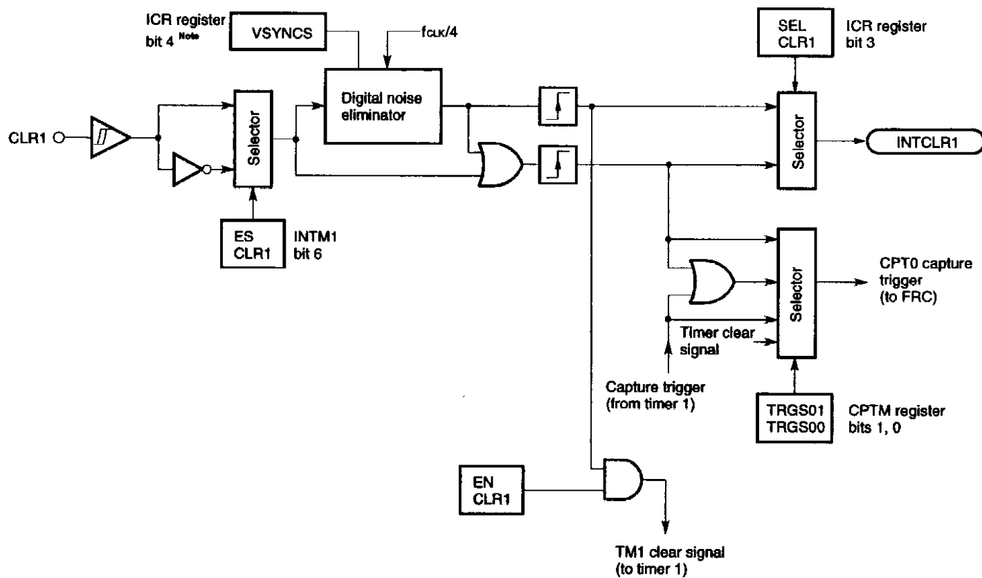
Fig. 3-13 Configuration of CLR1 Input Section★
