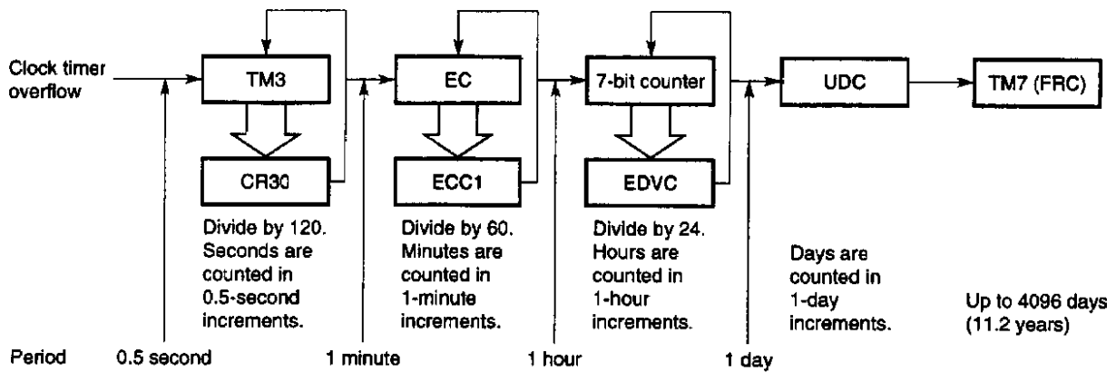
Fig. 3-23 Block Diagram of the Clock Function
